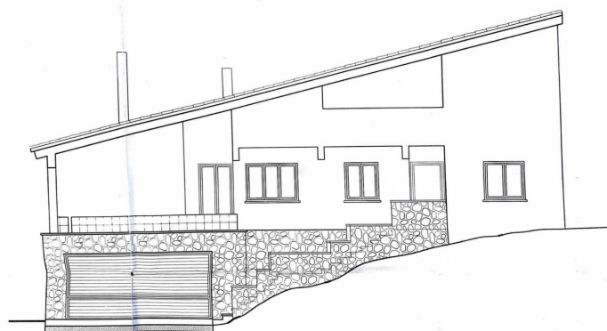
ALZADO PRINCIPAL
